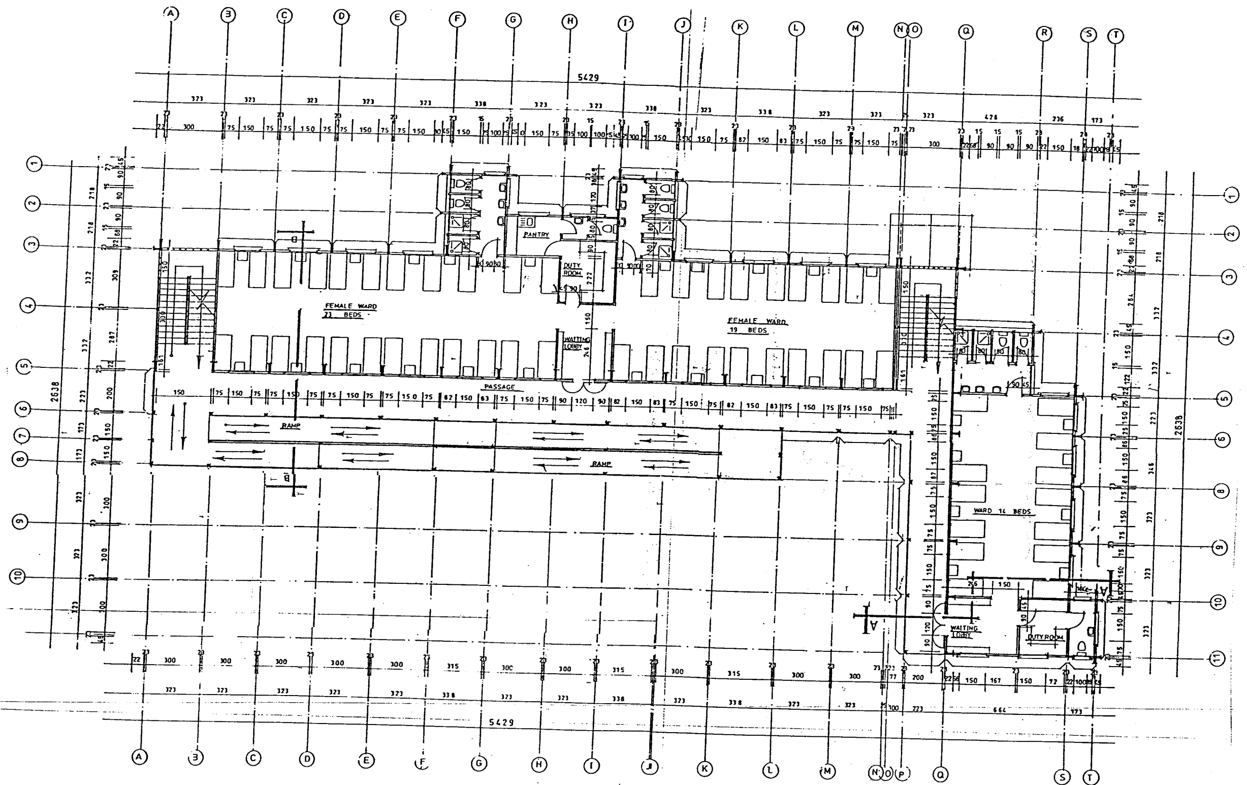
TYPICAL FIRST, SECOND AND THIRD FLOOR PLAN 1:100;
